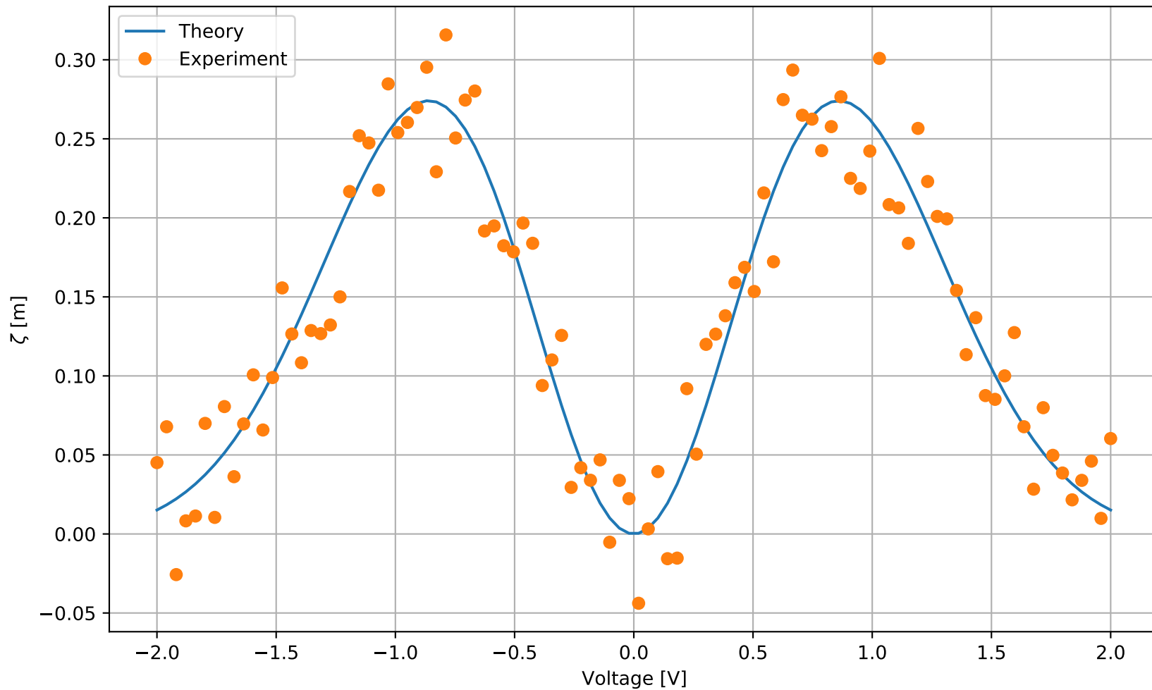
Nonsense graph
